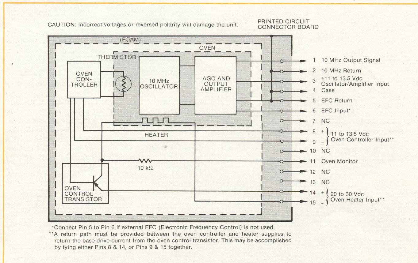
FIGURE 2 Block Diagram
